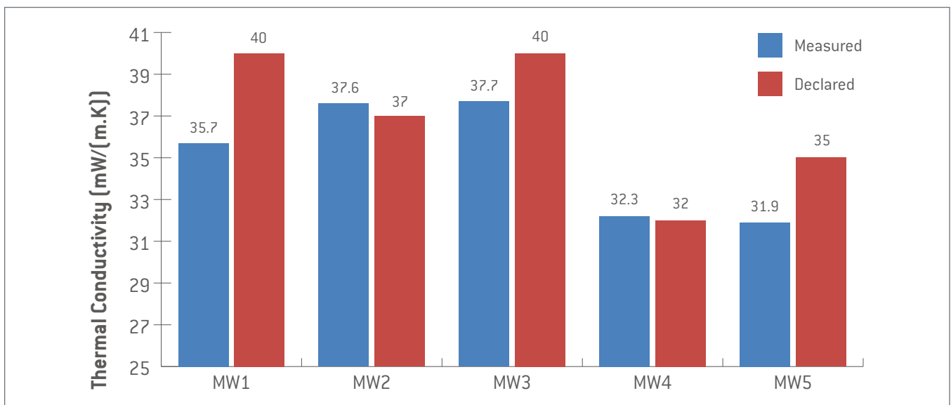
Summary of the thermal conductivity measurements (presented in blue) in comparison with available values of the corresponding product information sheets from the time of production (in red)
